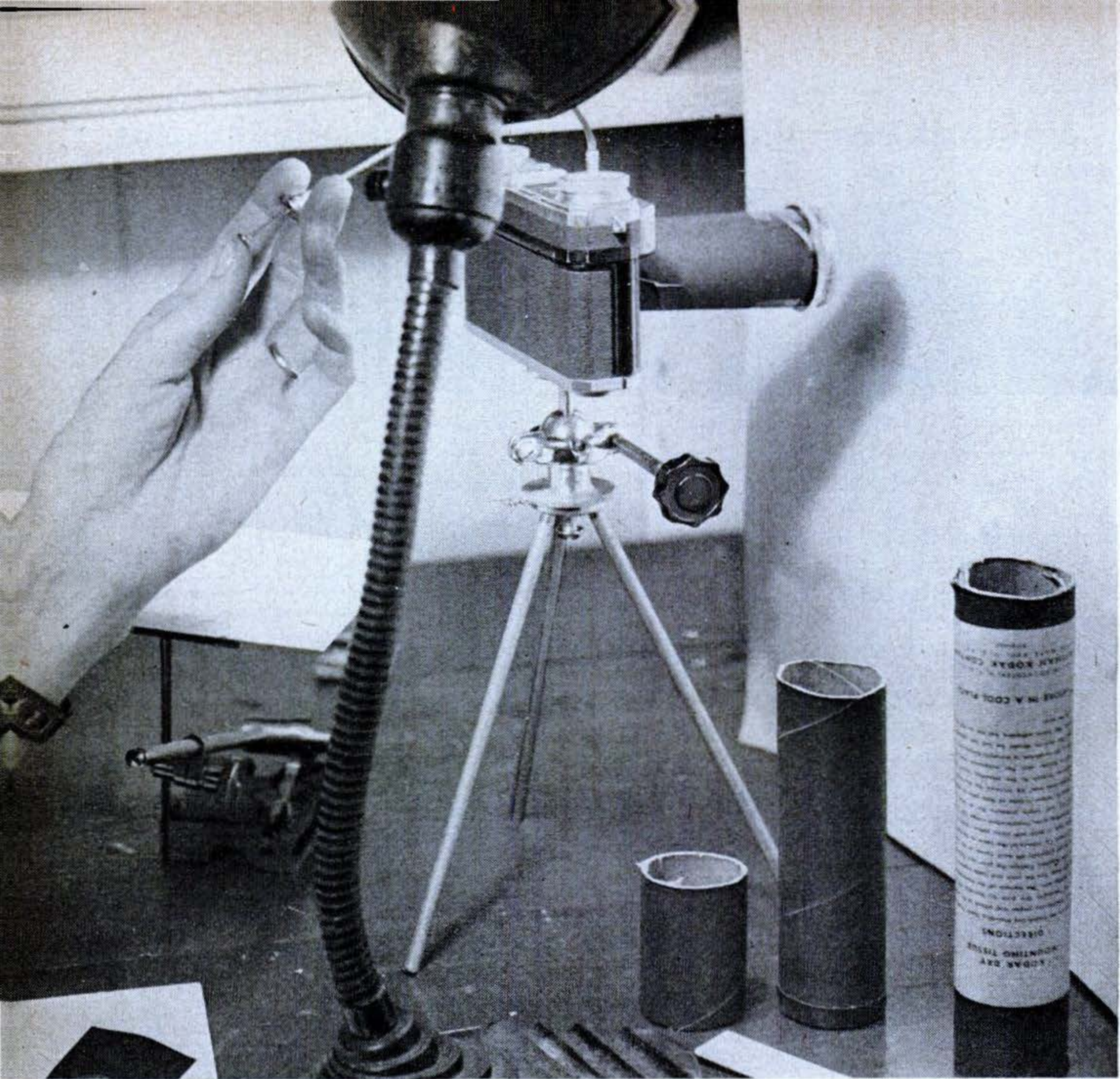
With this simple setup, you can photograph small objects at many times their original size.
